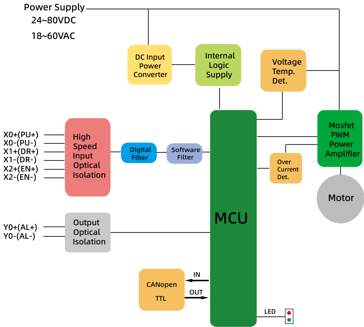
IG86EC Block Diagram
